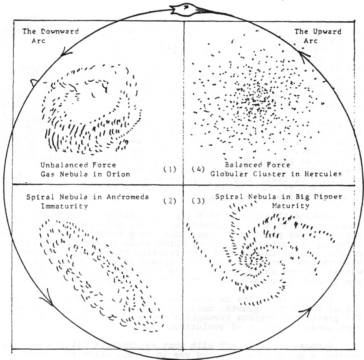
THE EVOLUTION OF A UNIVERSE
