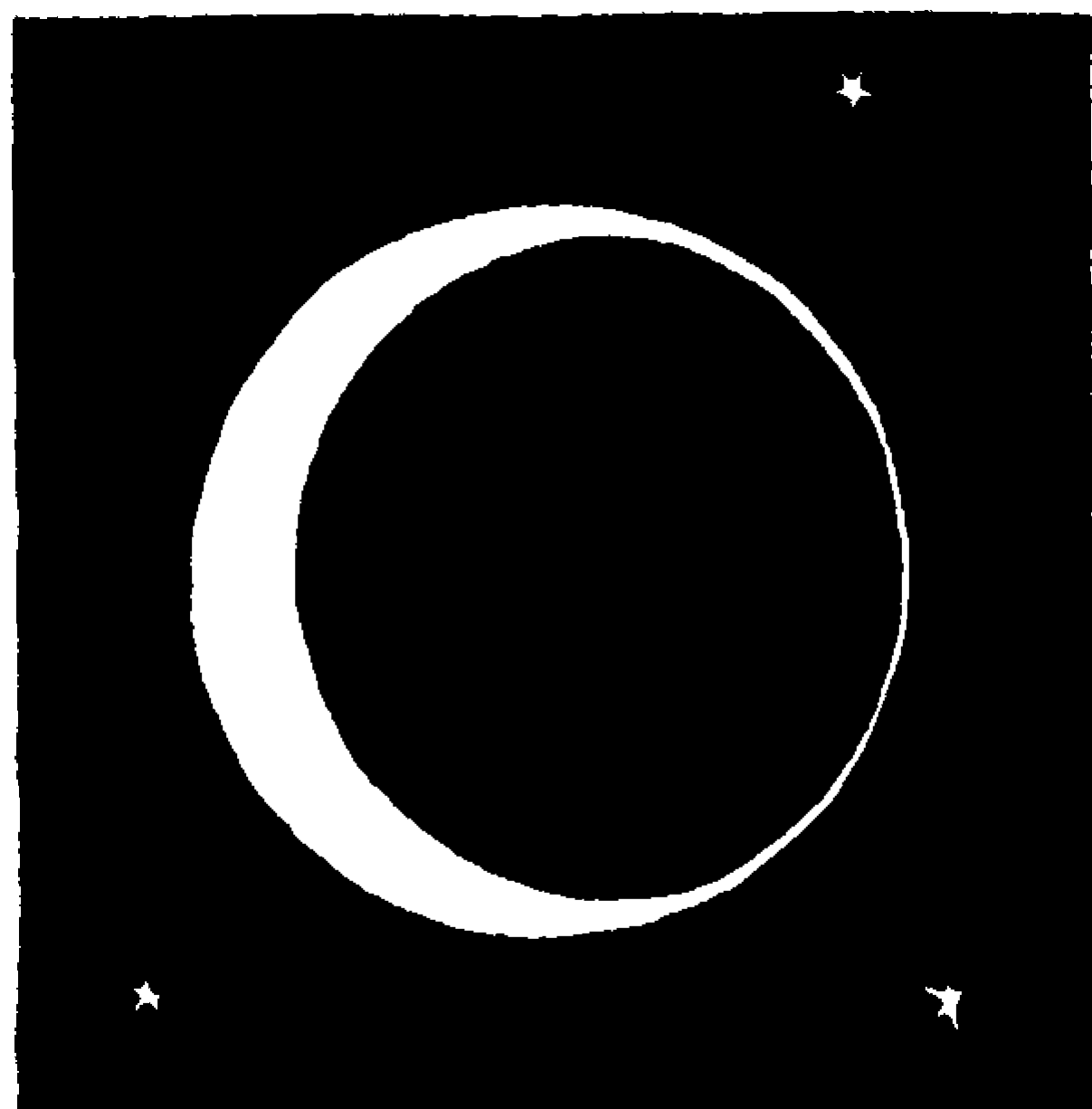
THE PLANET VENUS IN CRESCENT PHASE
