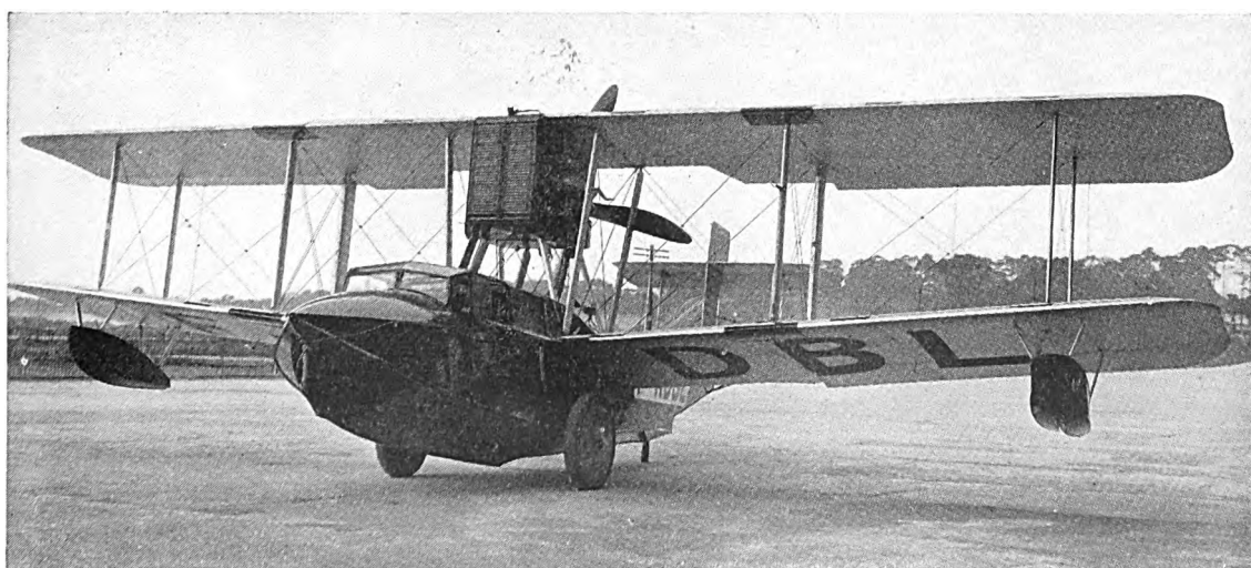
THE VICKERS "VIKING" AMPHIBIAN
