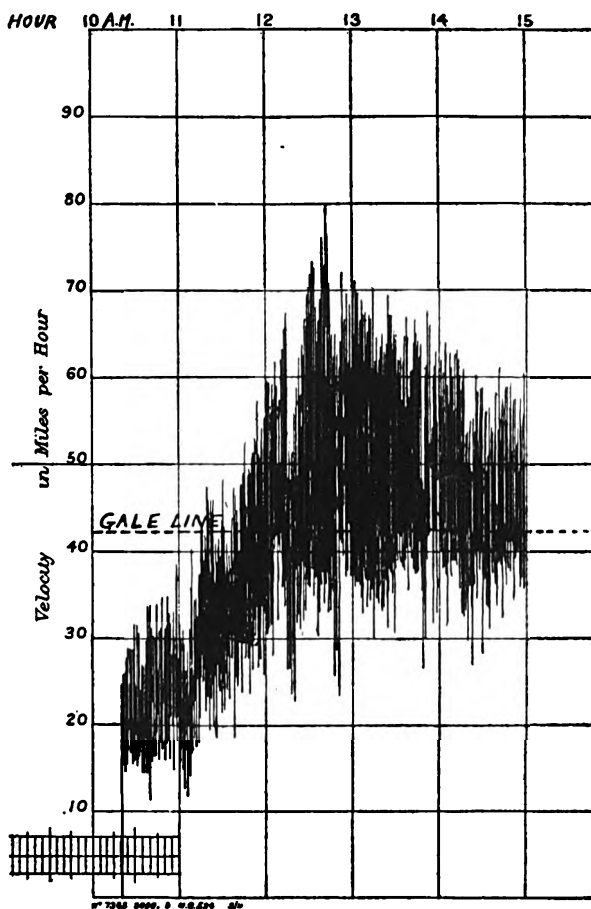
ILLUSTRATION OF A RECORD OBTAINED BY THE PRESSURE-TUBE ANEMOGRAPH DURING A GALE
