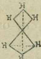
Ethane \text{C}_2\text{H}_6
