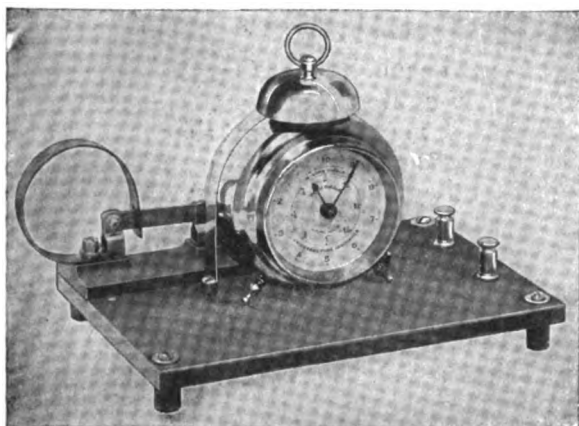
Fig. 193. Time Switch workt by an Interval Timer. These ar m'f'd. by Victor Electric Corporation, Chicago. These Time Switches I hav found to be indispensable for general electro-therapeutic use. They shut off the current when it is prearranged that they should and saves worry and time. These ar also made in a two-pole type.
