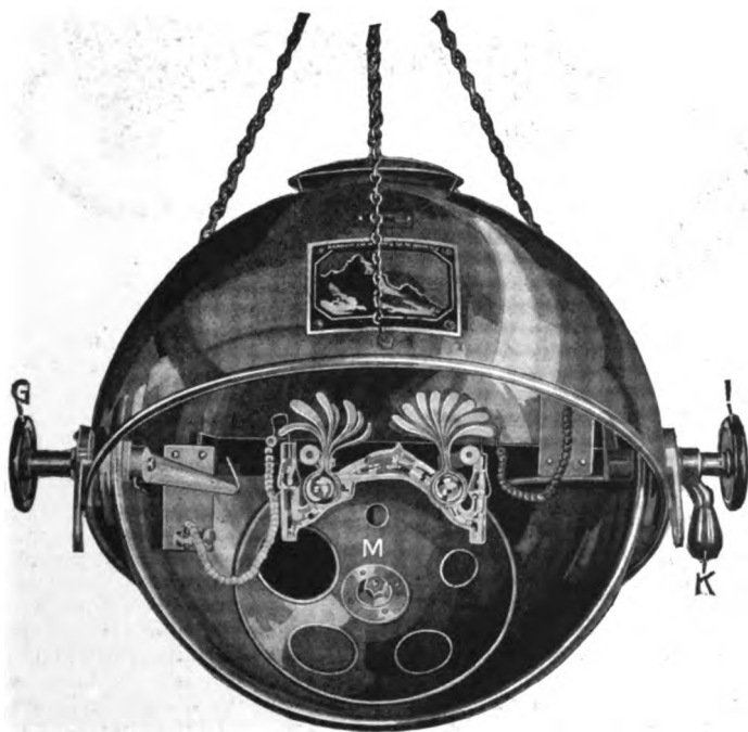
Fig. 180. Heraeus Sun Lamp with reflector lowered to show burner-tilting mecanism and reverse side of selectiv shutter. I is the tilting nob and K is the lock nut for same. G is at one end of the burner holder. M is the selection shutter.
