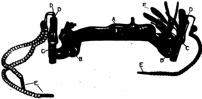
Fig. 179. A. C. Burner for the Heraeus Alpine Sun Lamp. A represents the mercury-vapor-arc tube, which is 5\frac{1}{2} inches long, with two positive electrodes and one negative electrode D .
