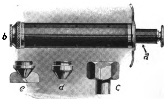
Fig. 276. CO 2 crayon outfit. See technic for using, Fig. 275.
