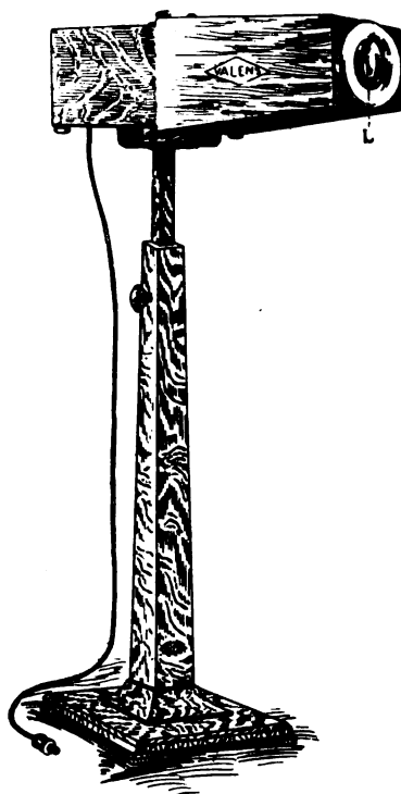
Fig. 106. Showing a projectoscope for holding several absorption cels at a time. With this apparatus I can make any color known. L represents the front Cel or hollow lens.
