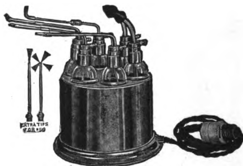
Fig. 393. This Heater is made of one piece of drawn brass, highly polisht and nickel plated. The top can be removed for adjusting the electric bulb. The bulb is of four-candle-power which wil keep the solutions at from 150 to 160 degrees Fahrenheit.
