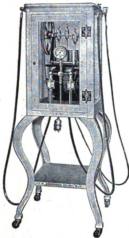
Fig. 152. The Sorensen Tankless Air Compressor Outfit No. 220.
