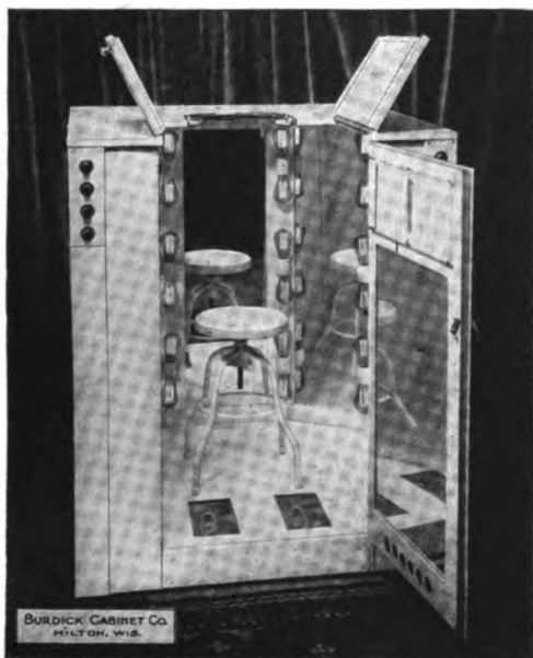
Fig. 162. Showing interior of same cabinet as shown in Fig. 161. Special enamelled reflectors are back of the scientifically placed lamps. I like enamel plates inside better than mirror plates. I believe more heat is radiated from the enamel plates.
