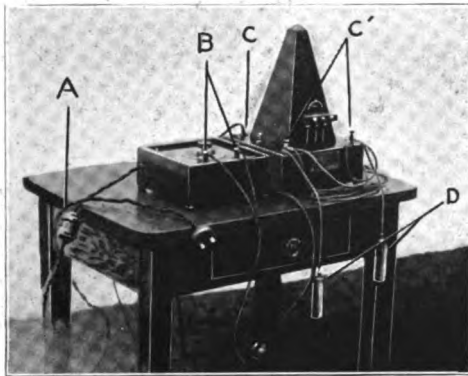
Fig. 249. Valens Metronomic Interrupter and the No. 1 Sinustat combined. Notis that the Sinustat has been removed from its original case and put into a form to match the Interrupter. This makes an elegant outfit. A is the feed current from the 110-volt lighting fixture. B ar the binding posts from which the controld current goes to the feed plug C of the Interrupter. C' ar the binding posts from which the Interrupted current goes to the patient electrodes of any kind D .
