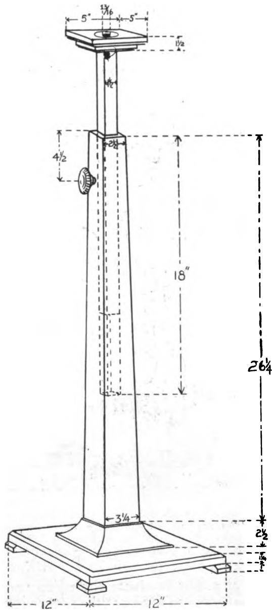
Fig. 118. Working plan of Valens Adjustable Pedestal. It should be made of quartered oak to match the Valens Bio-Dynamo-Chrome.
