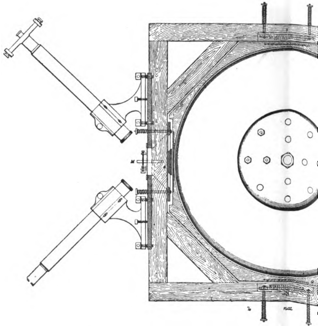
FIG 19 Plan of optical frame with steel disk in position, and glass panes in position. G represents one of the panes of optical glass. M represents one of the mirrors. The drawing shows the fixing of the four mirrors in the frame, each mirror held by a brass plate supported by three screws. It is pressed by the spring-bolts shown.
