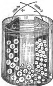
FIG. 16. Atoms of hydrogen marked + collected upon — copper, atoms of oxygen marked — set free at + zinc. Arrows show direction of current before polarization occurs.
