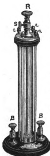
FIG. 51. HYDRO-RHEOSTAT. Height, 9\frac{1}{4} inches.
