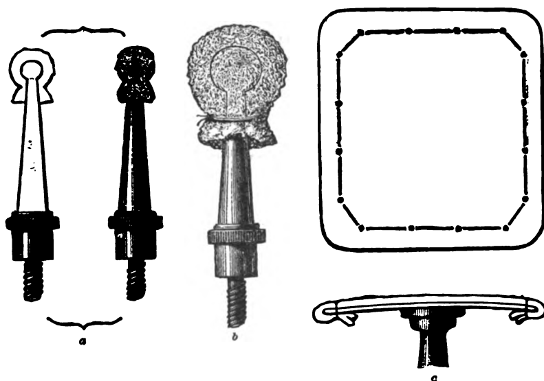
FIG. 6.—Various electrodes (natural size) which may be fastened to the handle represented in Fig. 7. a, "fine" or "smallest" electrode. b, "small" electrode. c, "medium" electrode, slightly convex upon the surface. All the electrodes are metallic and nickel plated, a and b covered with sponge, c, with flannel and linen.
