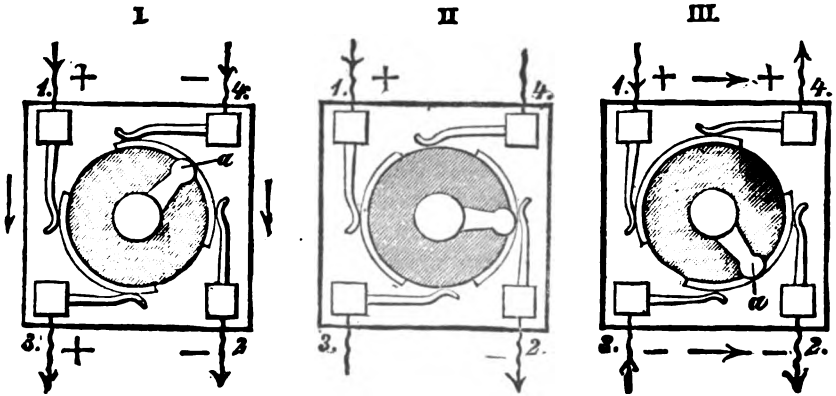
FIG. 5.—Schematic representation of the polarity changer in three different positions of the hard rubber disc, which may be revolved by the lever a . Contacts 1 and 2 are connected with the battery, 3 and 4 conduct the current into the circuit of closure. In I., the anode is situated at 3, in III. at 4, and the direction of the current in the circuit of closure is accordingly reversed. In II., the circuit is open.
