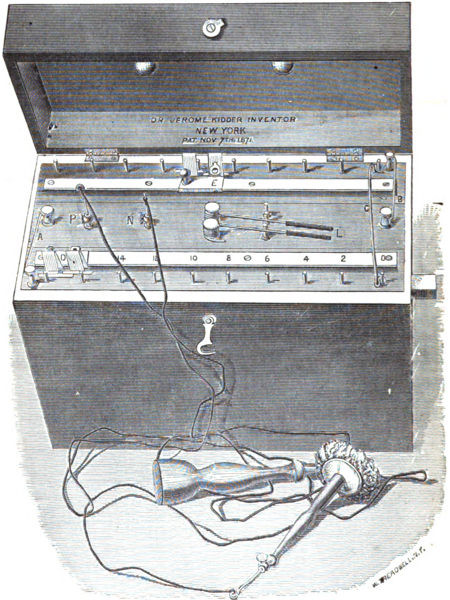
FIG. 51. Eighteen-cell zinc-carbon battery (Kidder).
