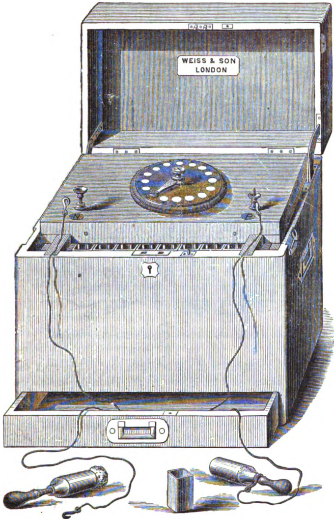
FIG. 81. Foveaux's Portable Galvanic Battery.
