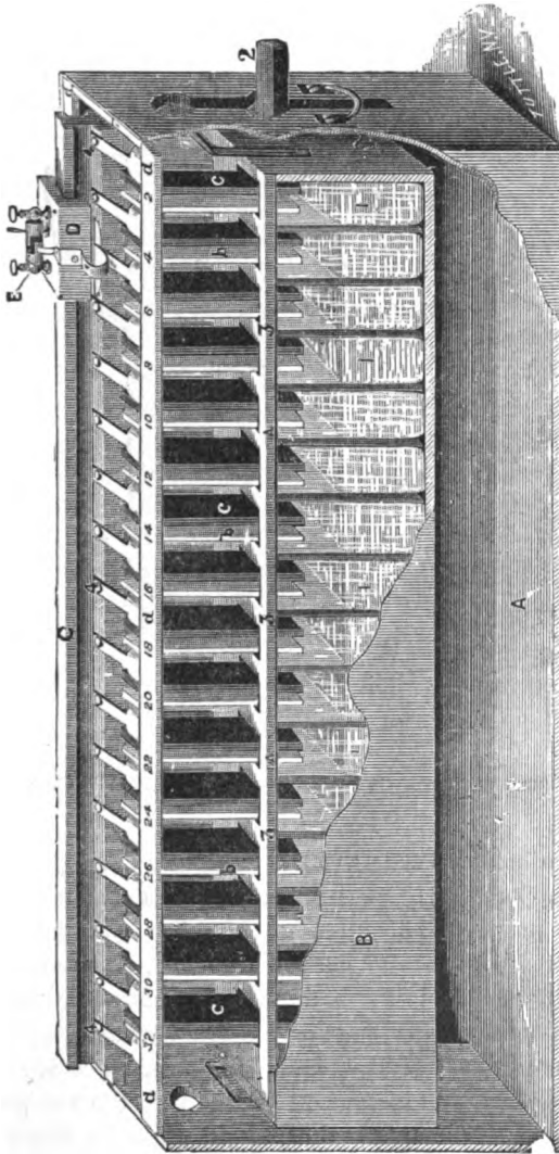
FIG. 48. Thirty-two cell zinc-carbon office battery, with slide, current interrupter and reverser, and hydrostat (Galvano-Faradic Manufacturing Company).
