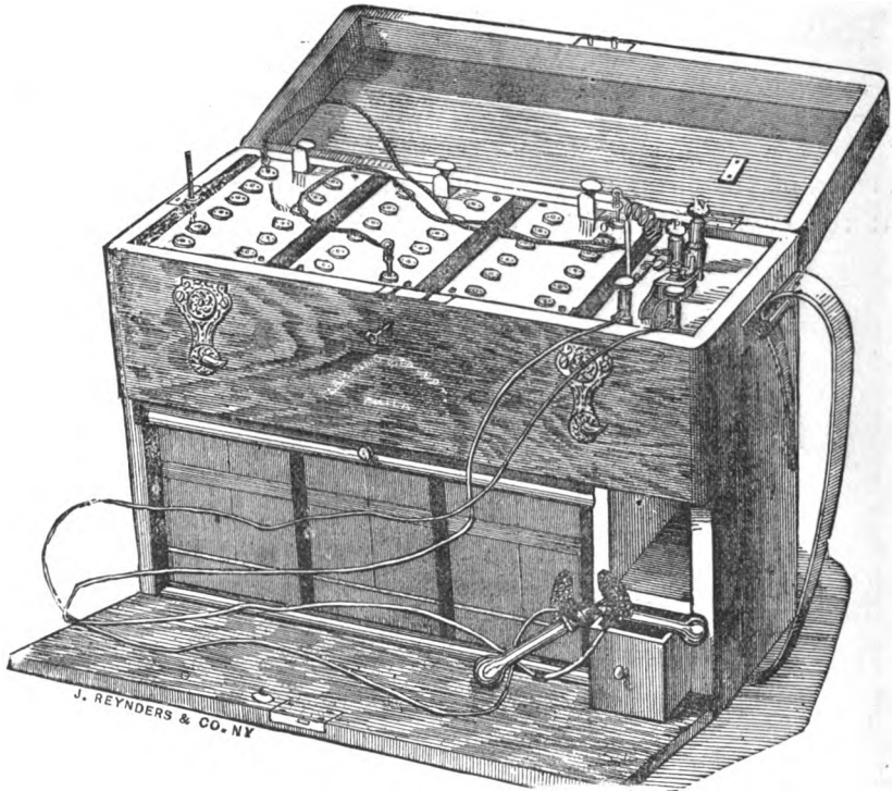
FIG. 9.—Thirty Cell Zinc-carbon Battery. (Fleming & Talbot.)
