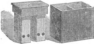
FIG. 22.—Kidder's Galvano-Cautery Battery.
