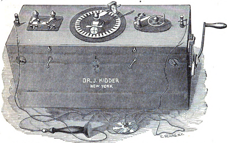
FIG. 7.—Thirty-six Cell large Zinc-carbon Galvanic Battery, with Circular Switch, Reverser, and Interrupter, for Office or Hospital Use. (Kidder.)
