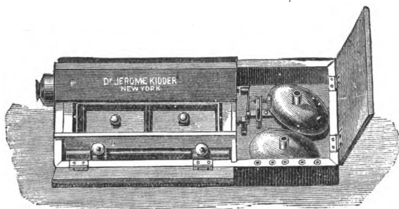
FIG. 14.—Modification of Gaiffe's Faradic Apparatus. (Kidder.)
