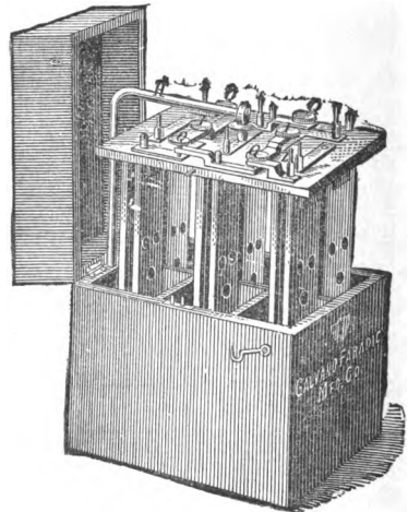
FIG. 23.—Piffard's Galvano-Cautery Battery.
