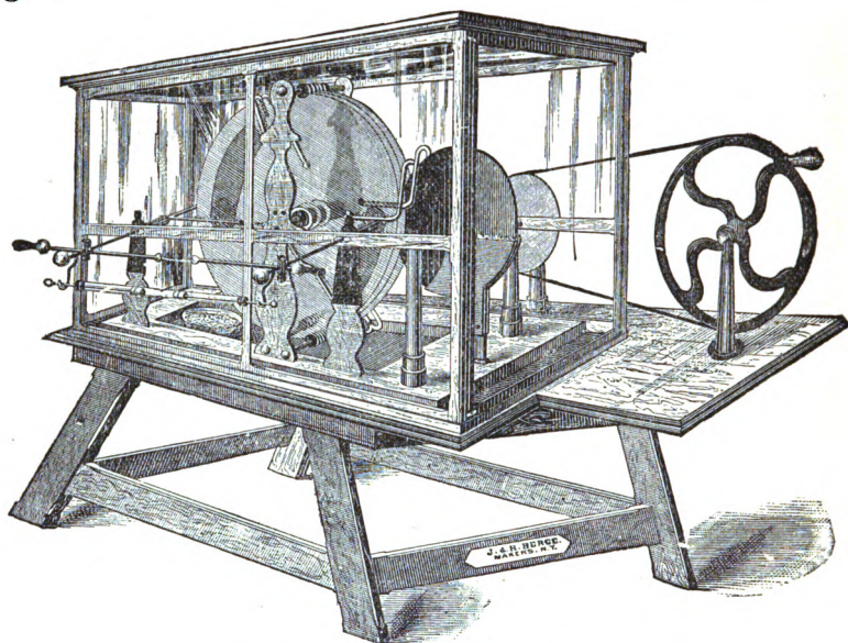
FIG. 1.—Apparatus for Franklinization.
