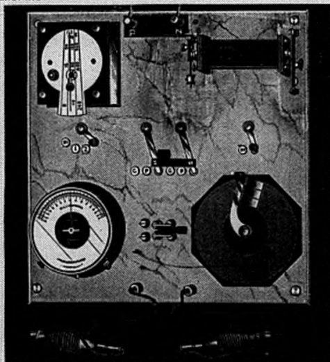
McINTOSH No. 6 OFFICE PLATE
