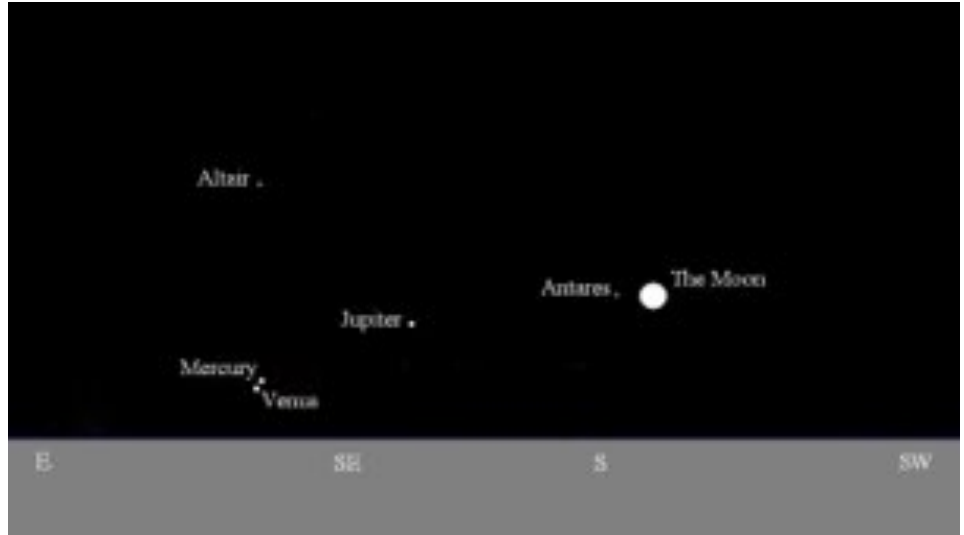
February 28th 2008 before sunrise, looking southeast. The two innermost planets close together in the sky is a relatively rare sight.
