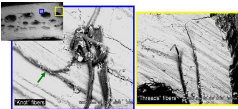
Scanning Electron Microscope (SEM) images of SC bone. Top Left image's squares are around two different kinds of "fibers" seen individually under higher magnification in larger photos below.
