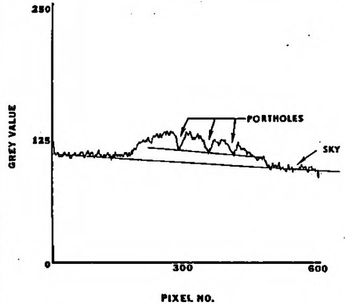
Figure 1: Computer-generated image-density profile across the UFO-like object depicted in photograph number 5. Note: this scan is a mirror-image of the photograph, in which the right side of the diagram corresponds to the left side of the photograph. Image brightness increases from black at the bottom of the chart to white at the top.
