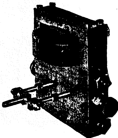
Fig. 6. Unique Alternating Current Generator for exciting Tesla's early "Beat" Receptor. Actuated by Compressed Air or Steam Which Vibrates a Special Diafram-Coil.
