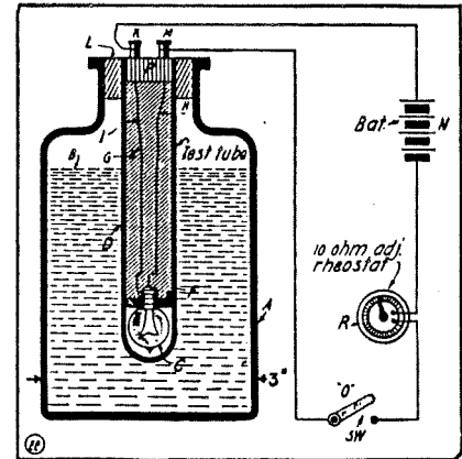
Dark-room Lamp Made from Battery Lamp, Test Tube and Red Solution.
