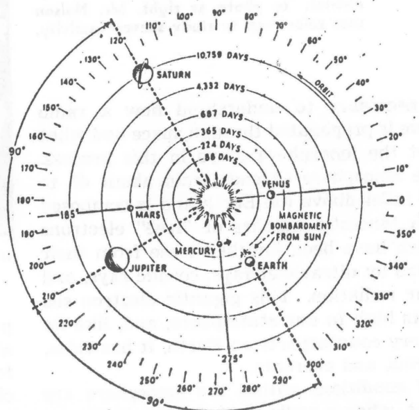
Fig. 2. When Saturn, Jupiter, and the Earth are at 90^\circ to each other, magnetic storms appear on Earth and radio reception is poor. Drawing on page 45 is artist's conception of this relationship.
