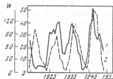
FIGURE 5. Dynamics of morbidity (1:10,000 pop.) with scarlet fever in Leningrad (1), after Ioffe et al. /31/, and curve of solar activity (2)
