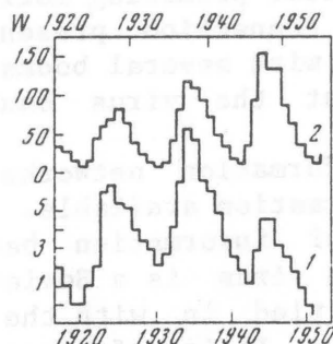
FIGURE 10. Dynamics of malaria in USSR (after Sergiev et al.) and solar activity:
