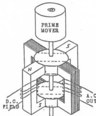
Peter Lindemann's Variable Reluctance Generator
