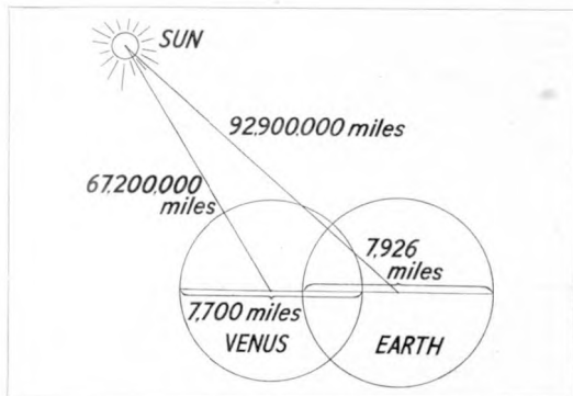
Venus and the Earth compared.
